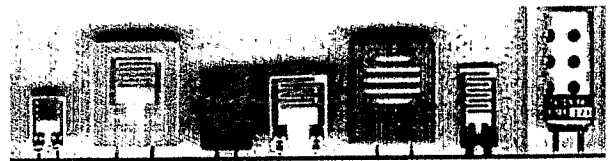
Photo 2. Resistive sensors are based on an interdigitated or bifilar winding. After deposition of a hygroscopic polymer coating, their resistance changes inversely with humidity. The Dunmore sensor (far right) is shown 1G size.
