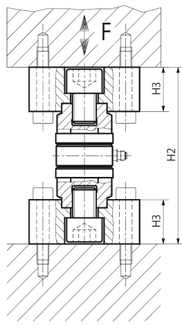
Fig. 2 Force link with flanges fitted on both sides. Insert for compression force loading.
