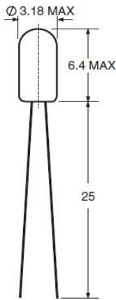
T-1 Wire Lead
