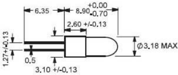
Bi-Pin
