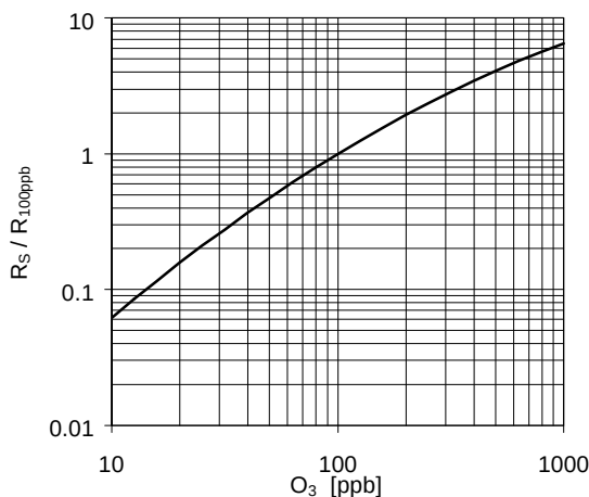
Figure 1: R_S / R_{100\text{ppb}} as a function of gas concentration at 50% RH and 25^\circ\text{C} .
