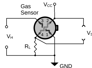
Figure 3: Measurement circuit for \text{O}_3 detection.
