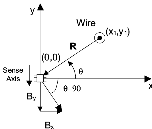
Figure 7—Sensing the position of a wire
