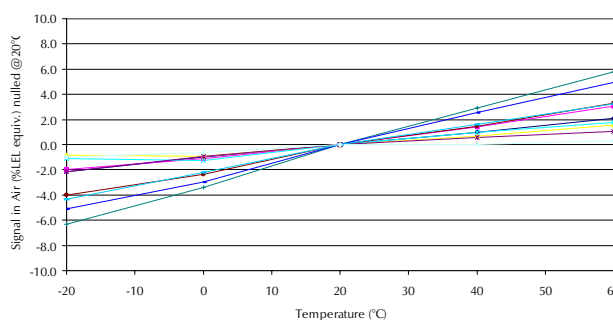
Effect of Temperature on Zero Signal
