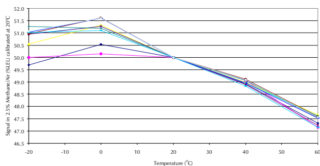
Effect of Temperature on Methane Signal
