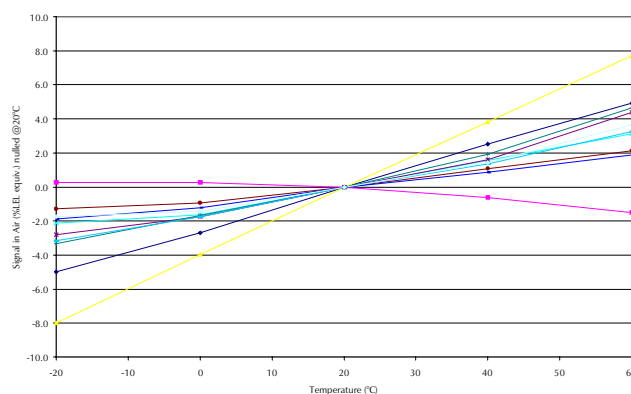
Effect of Temperature on Zero Signal
