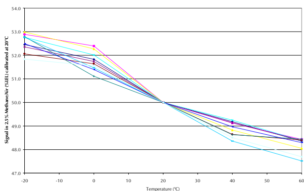
Effect of Temperature on Methane Signal
