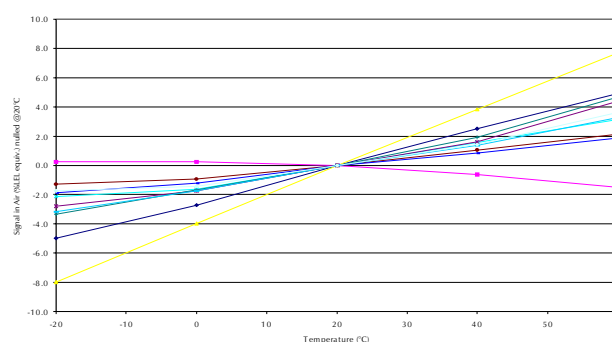
Effect of Temperature on Zero Signal
