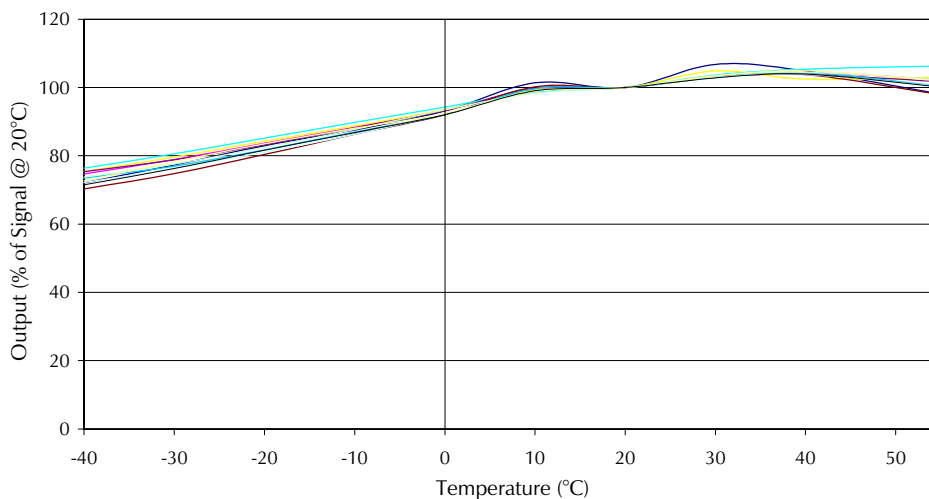
4ND Nitrogen Dioxide CiTiceL - Baseline vs Temperature
