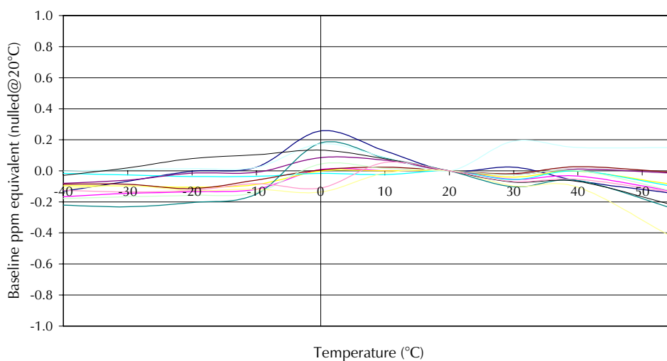
4ND Nitrogen Dioxide CiTiceL - Baseline vs Temperature
