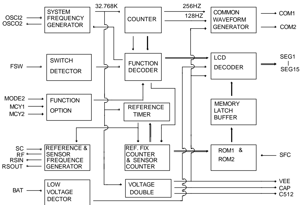
BLOCK DIAGRAM
