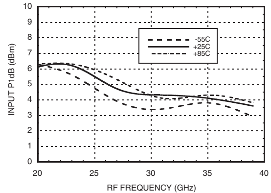
P1dB vs. Temperature @ LO = +12 dBm
