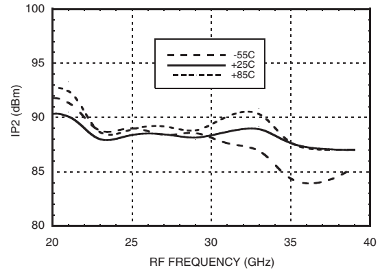
Input IP2 vs. Temperature @ LO = +12 dBm
