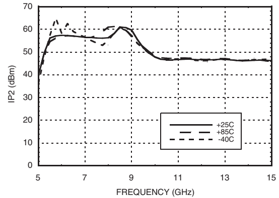
Input IP2 vs. Temperature @ LO = +15 dBm *
