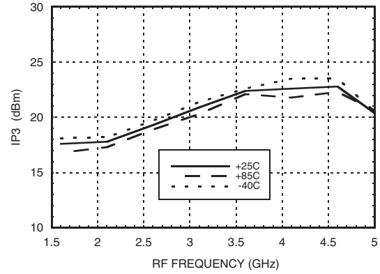
Single Channel: Input IP3 vs. Temperature @ LO = +13 dBm
