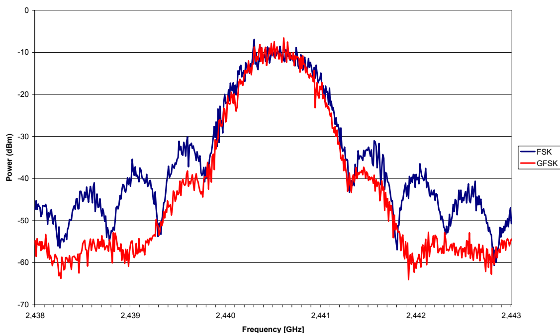
Figure 18. Modulated spectrum
