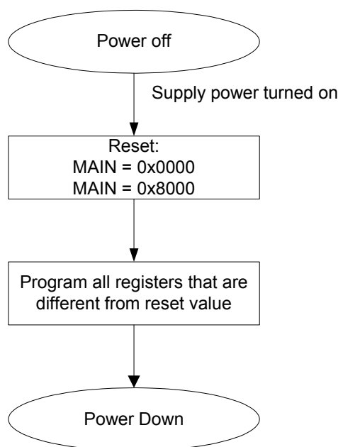
Figure 16. Initializing sequence
