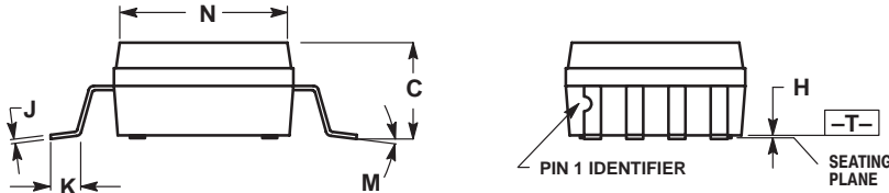
CASE 482-01 ISSUE 0
