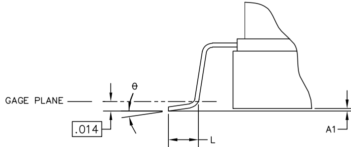
DETAIL "G"
