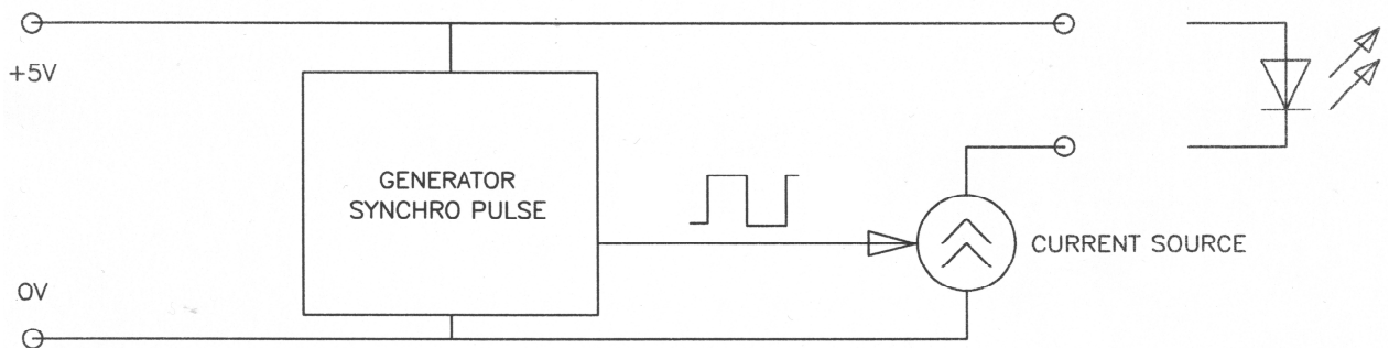
Fig.2. The Block diagram of mD-1c.
