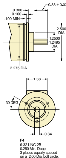
H25E - 2.50 Servo Mount
