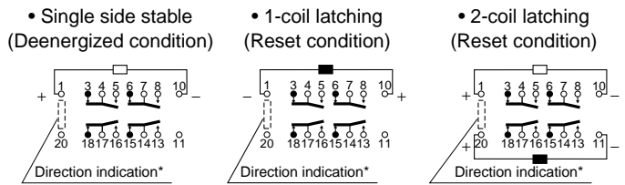
Schematic (Bottom view)
