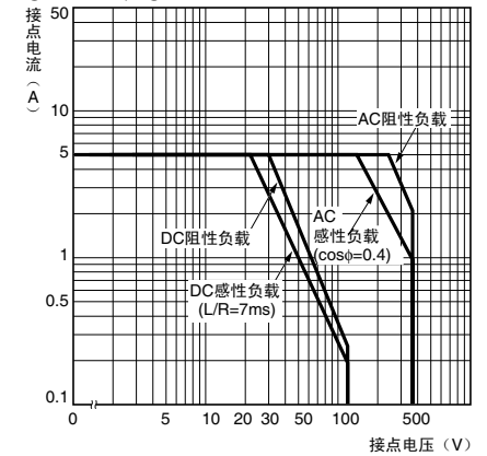
G2R-1-Z、G2R-1A-Z
