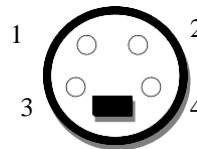
Figure 1 DFT-200 Connector
