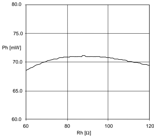
Fig. 3: P_h as a function of R_h . R_{series} = 88 \Omega and V_{cc} = 5 V
