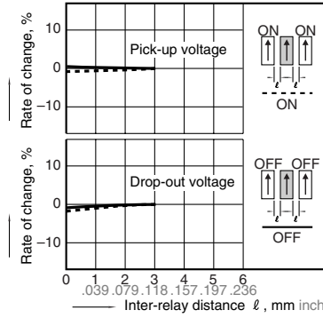
Change of pick-up and drop-out voltage (mounting by IRS method)
