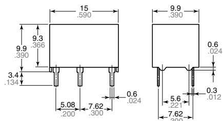
External dimensions
