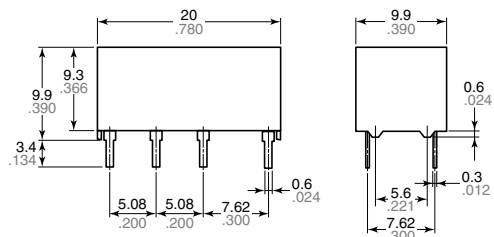
External dimensions
