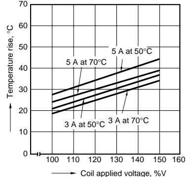
4-(1). Coil temperature rise (1 Form A type)
