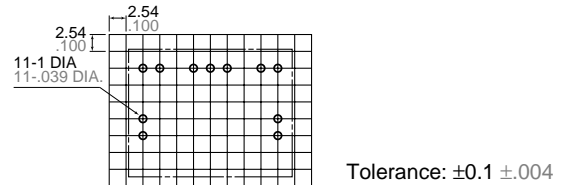
Schematic (Bottom view)
