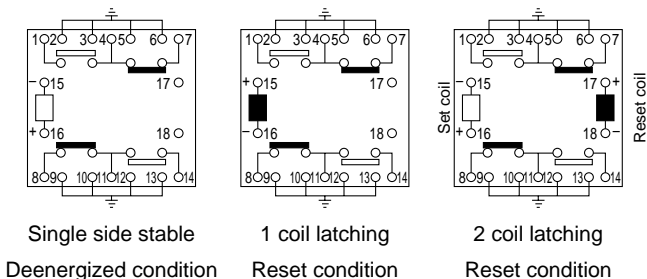
Schematic (Bottom view)
