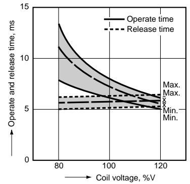
4-(3). Operate and release time (Without diode) (2C) RG2-12V 6 pcs.
