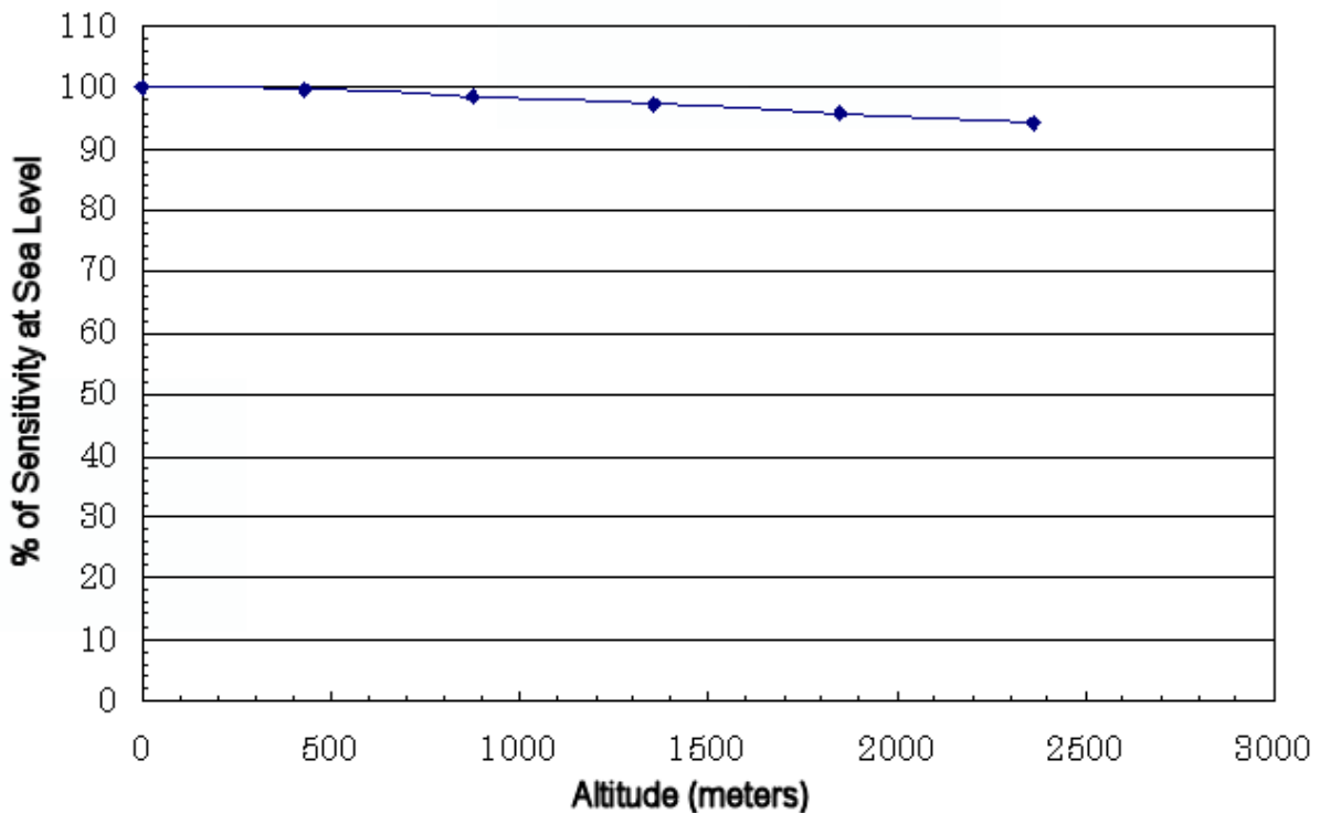
Effect of Altitude on Sensitivity, NAP-505
