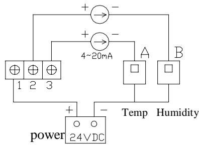
4-20mA output
