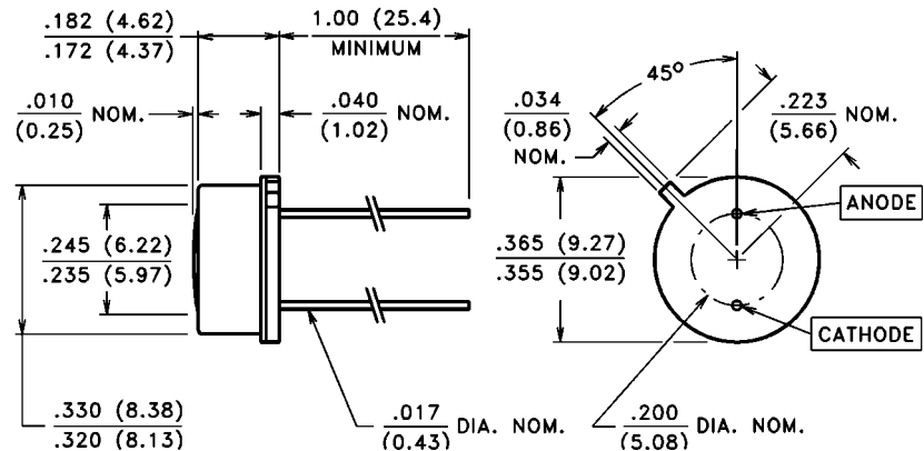
CASE 14 TO-5 HERMETIC CHIP ACTIVE AREA: .012 in 2 (7.45 mm 2 )
