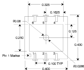
SM5410/SM5450 with Hole (Top View)
