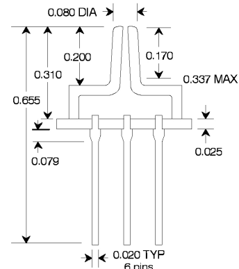
SM5410/SM5450 with Port (Side View)
