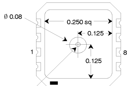
SM5310 with Port (Top View)
