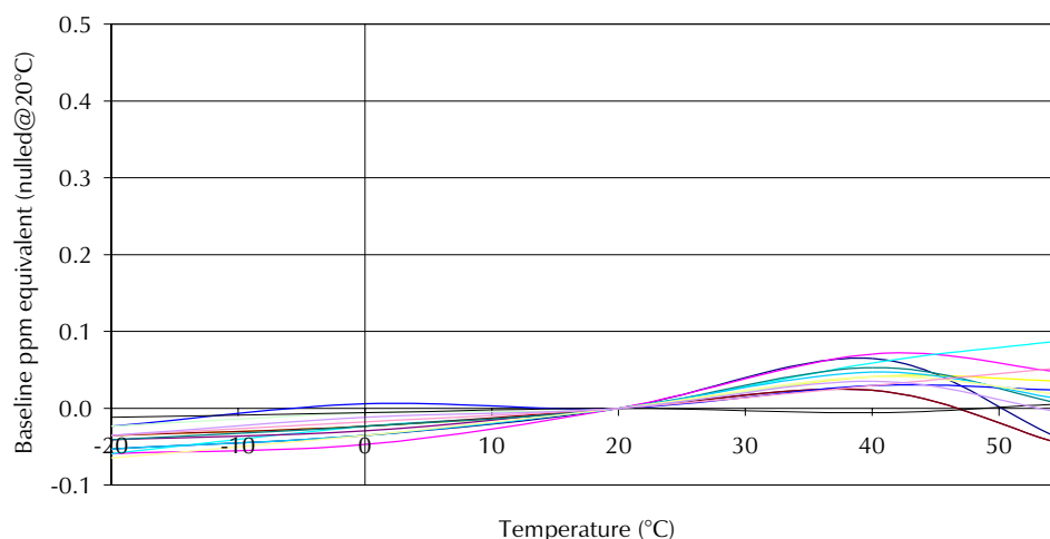
4PH Phosphine CiTiceL - Baseline vs Temperature
