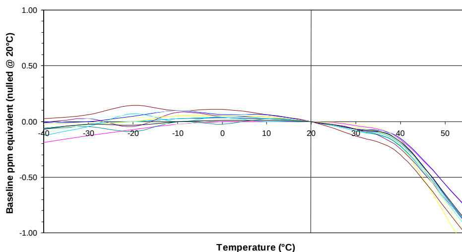
7H Hydrogen sulphide CiTiceL - Baseline vs Temperature
