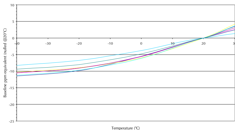
A7AM Ammonia CiTiceL - Baseline vs Temperature
