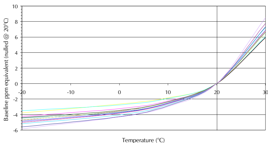
7AM Ammonia CiTiceL - Baseline vs Temperature
