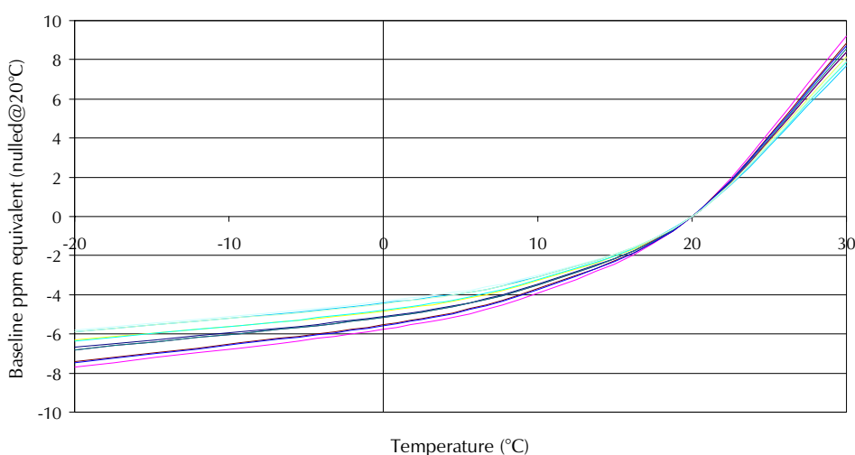
4AM Ammonia CiTiceL - Baseline vs Temperature
