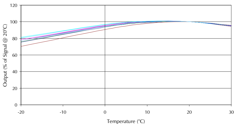
4AM Ammonia CiTiceL - Output vs Temperature
