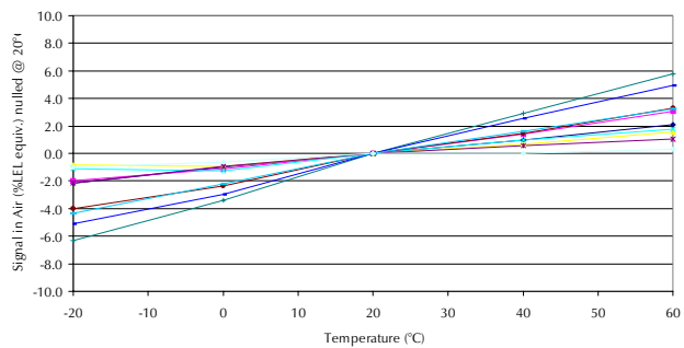
Effect of Temperature on Zero Signal
