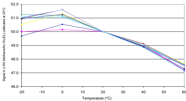
Effect of Temperature on Methane Signal
