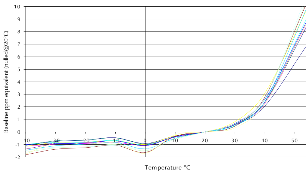
4NT Nitric Oxide CiTiceL - Baseline vs Temperature
