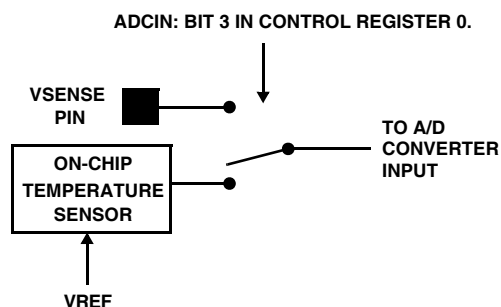
FIGURE 7. A/D CONVERTER INPUT SELECT STRUCTURE
