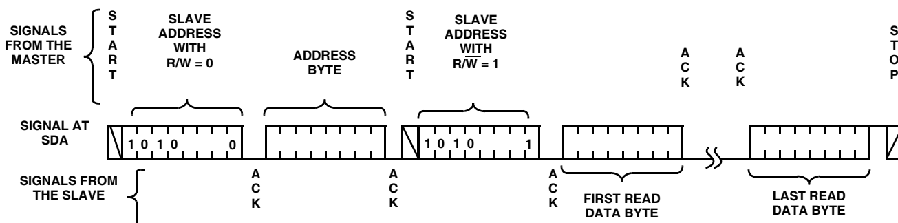
FIGURE 22. READ SEQUENCE
