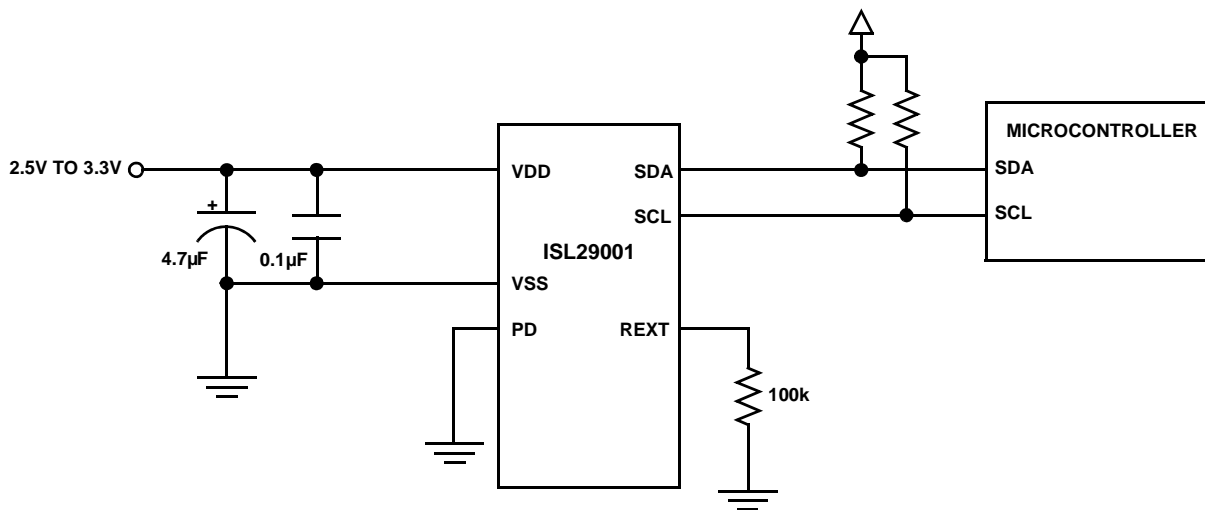
FIGURE 14. TYPICAL CIRCUIT
