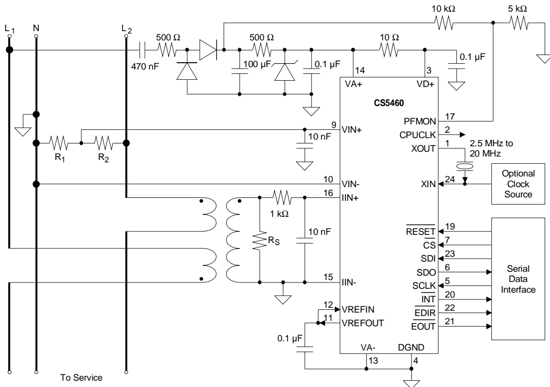
Figure 2. Typical Connection Diagram (One-Phase 3-Wire)
