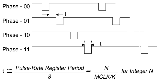
Figure 6. Multi-Phase System.
