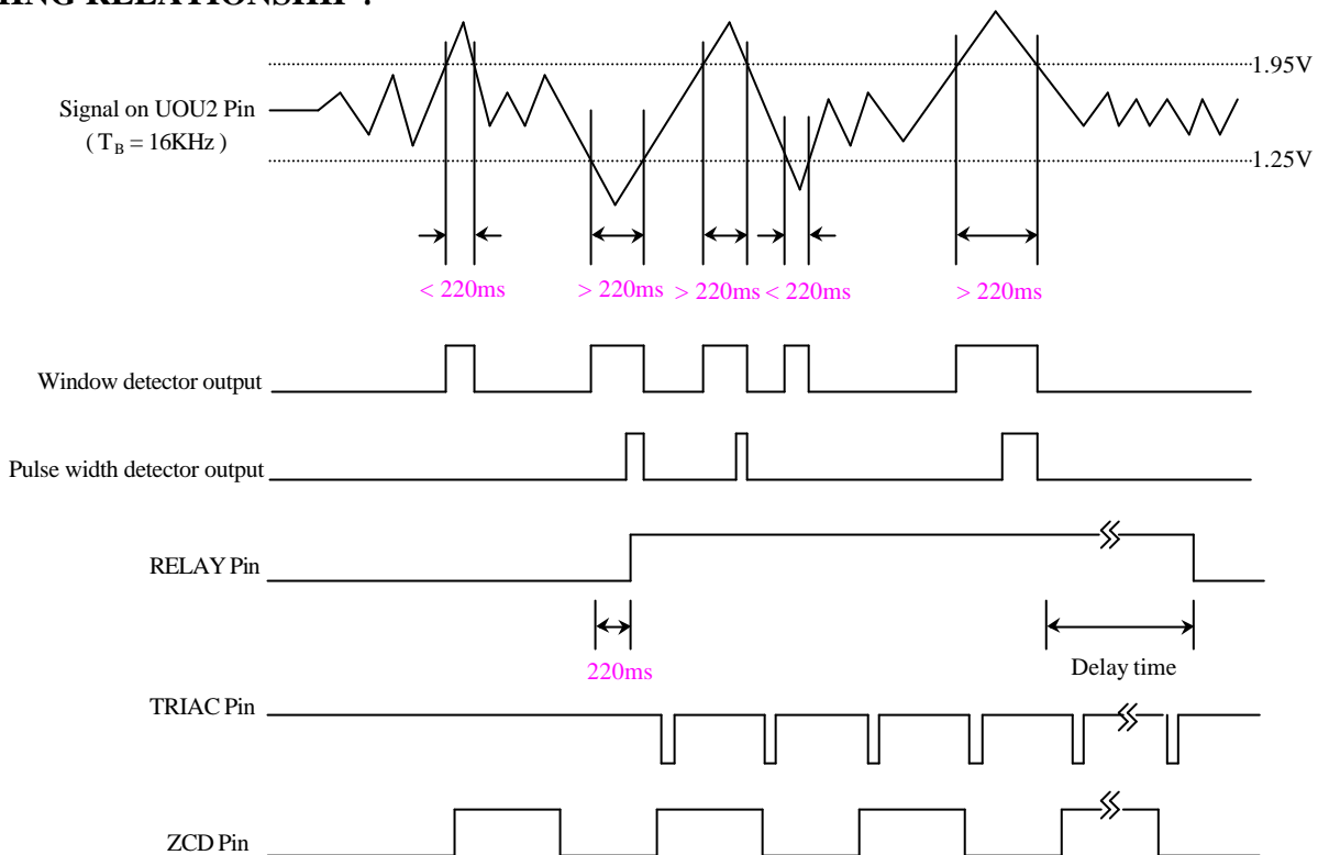
TIMING RELATIONSHIP :
